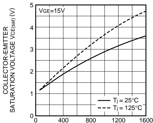
COLLECTOR-EMITTER SATURATION VOLTAGE CHARACTERISTICS (TYPICAL)
