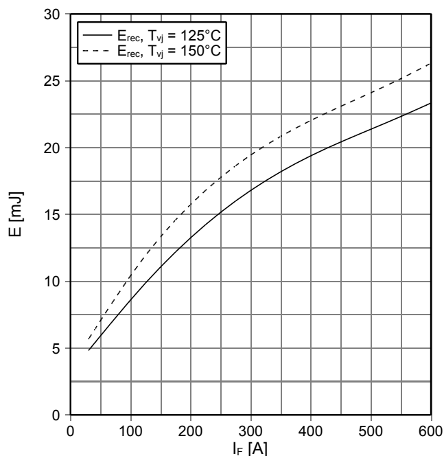
Schaltverluste Diode D1 / D4 (typisch) switching losses Diode D1 / D4 (typical) E_{rec} = f(I_F) R_{Gon} = 1.5 \Omega, V_{CE} = 300 V
